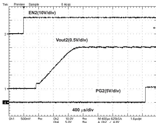
Figure 11. VO2=1.5V, PG2
