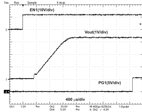
Figure 10. VO1=3.3V, PG1
