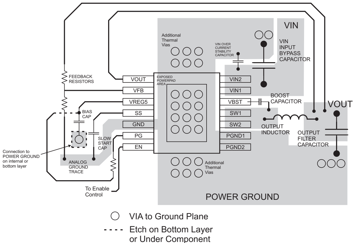
Figure 15. PCB Layout
