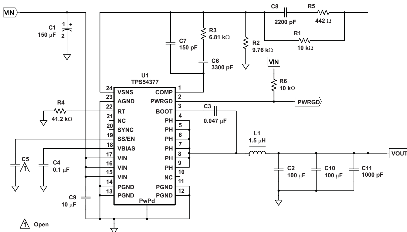
Figure 10. TPS54377 Schematic
