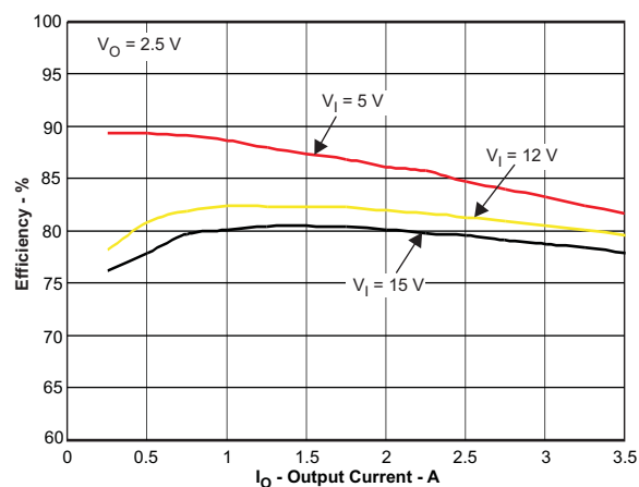
Figure 14. TPS54332 Efficiency
