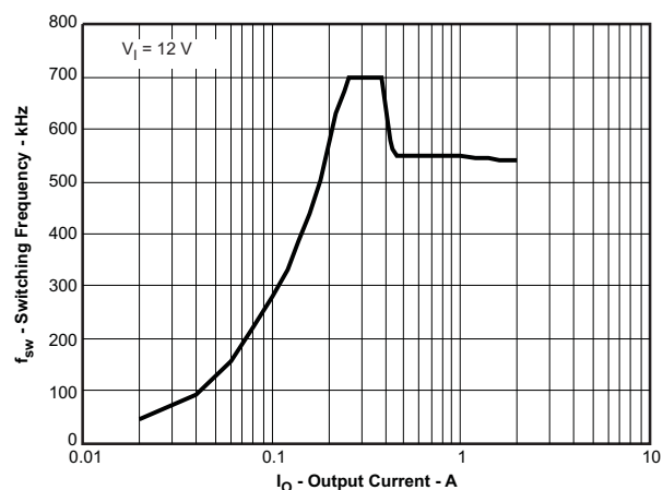
Figure 19. VO2=1.5\text{V} , SW-frequency vs Output Current
