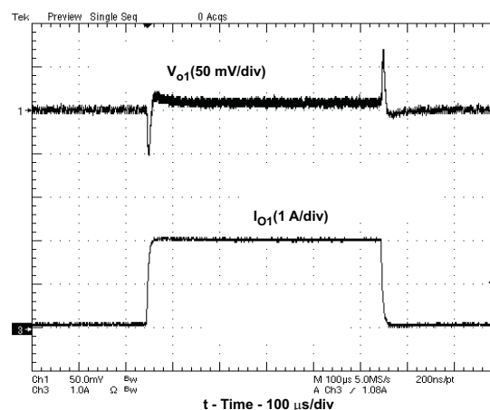
Figure 8. \text{VO1}=3.3\text{V} , 0A to 2A Load Transient Response
