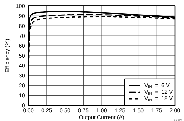
Figure 10. VO1=3.3V, PG1
