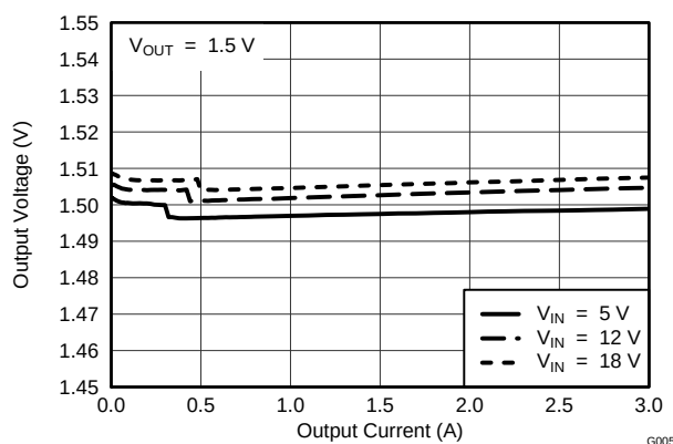
Figure 5. VO2=1.5V Output Voltage vs Output Current
