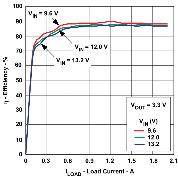
Figure 41. 3.3-V Output Efficiency vs. Load Current
