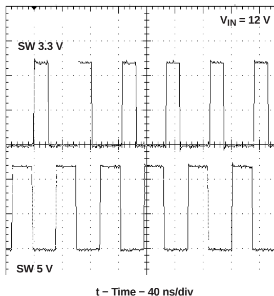
Figure 39. Switching Node Waveforms
