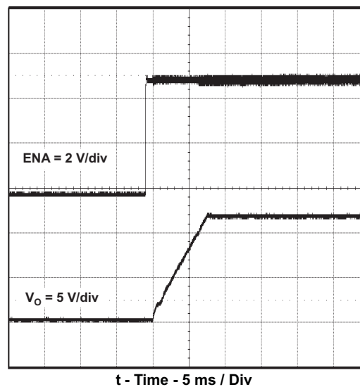
Figure 20. Startup Waveform, ENA and V_O
