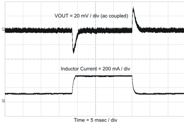
Figure 51. Load Transient
