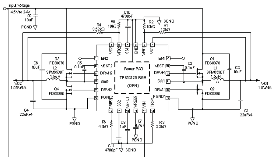
Figure 1. QFN
