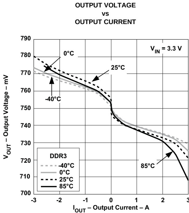
Figure 6. DC Regulation
