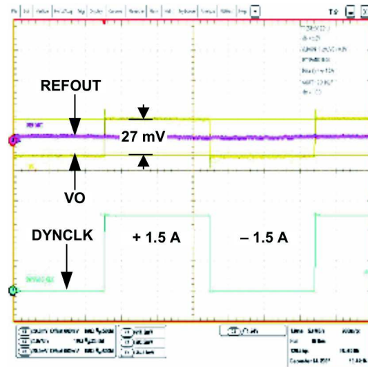
Figure 7. Transient
