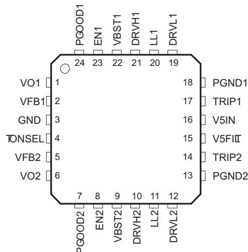
QFN PACKAGE (TOP VIEW)
