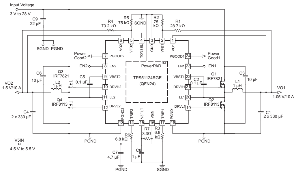
Figure 25. Typical Application Circuit
