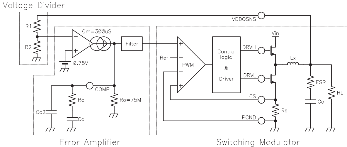
Figure 2. Linearizing the Modulator
