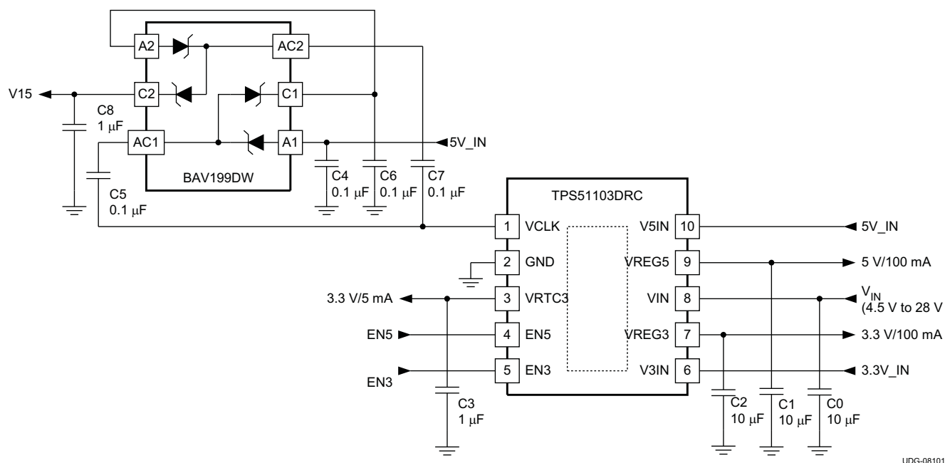
Figure 2. Typical Application
