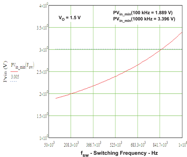
Figure 17. PV_{\text{IN}} vs Frequency
