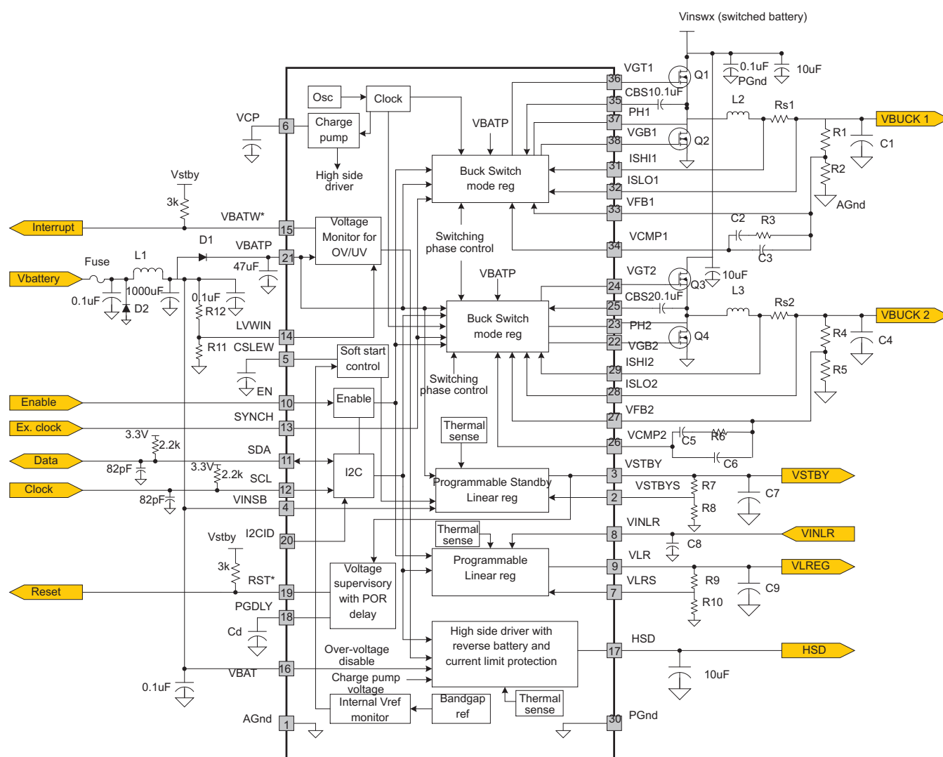
Figure 7. Typical Application Schematic
