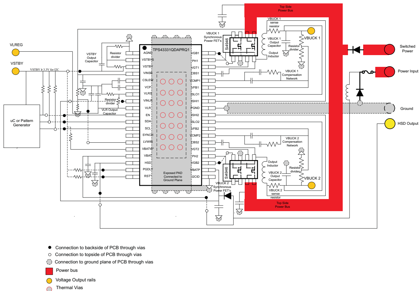
Figure 41. PCB Layout
