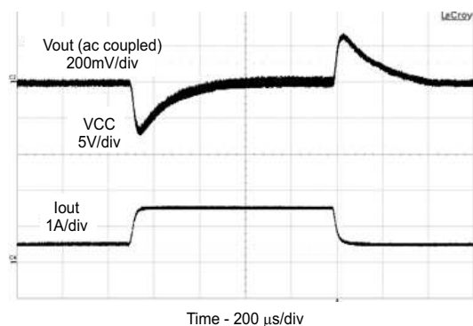
Figure 22. Load Transient
