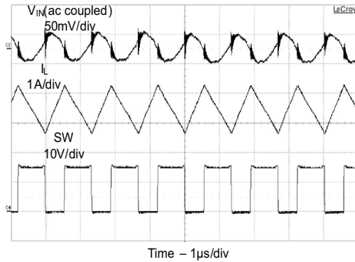
Figure 28. Input Ripple in CCM
