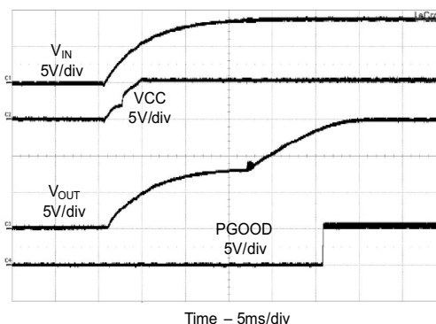
Figure 23. Start-up with VIN
