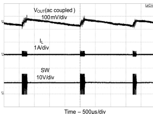
Figure 27. Output Ripple in Pulse-Skipping Mode
