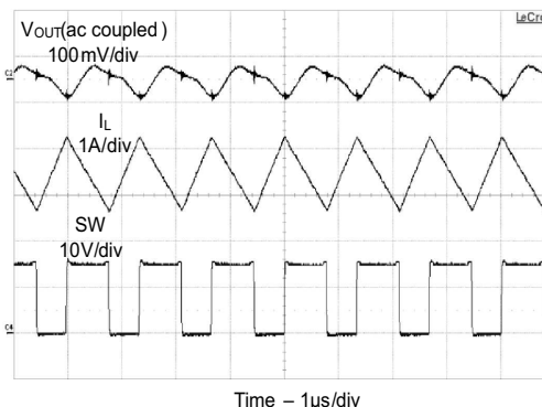
Figure 25. Output Ripple in CCM
