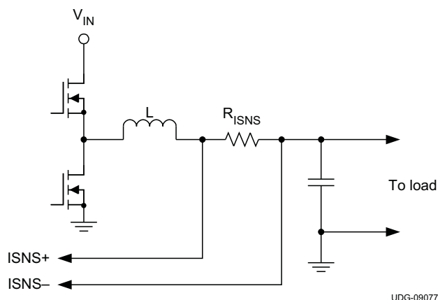
Figure 19. Current Sensing Using Sense Resistor
