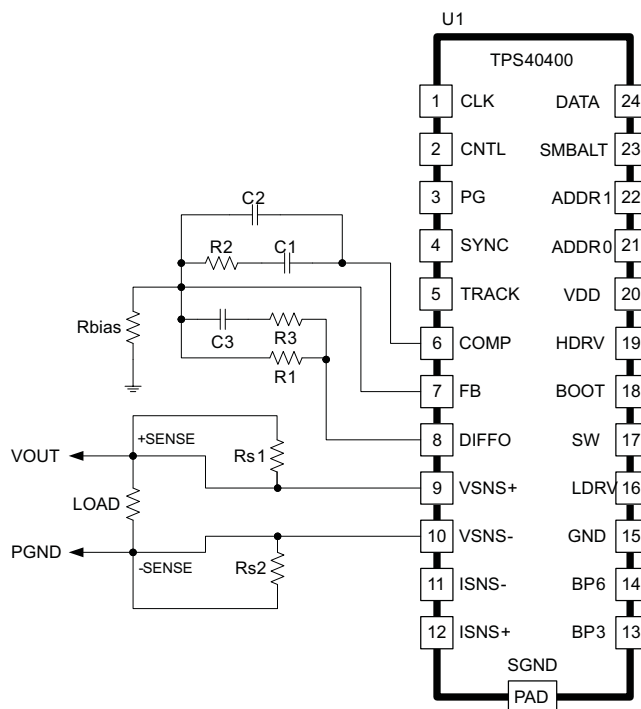
Figure 22. Remote Sense Schematic
