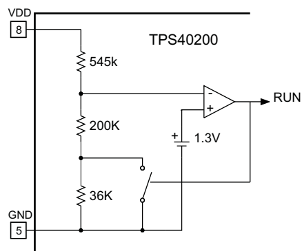
Figure 30. Undervoltage Lockout
