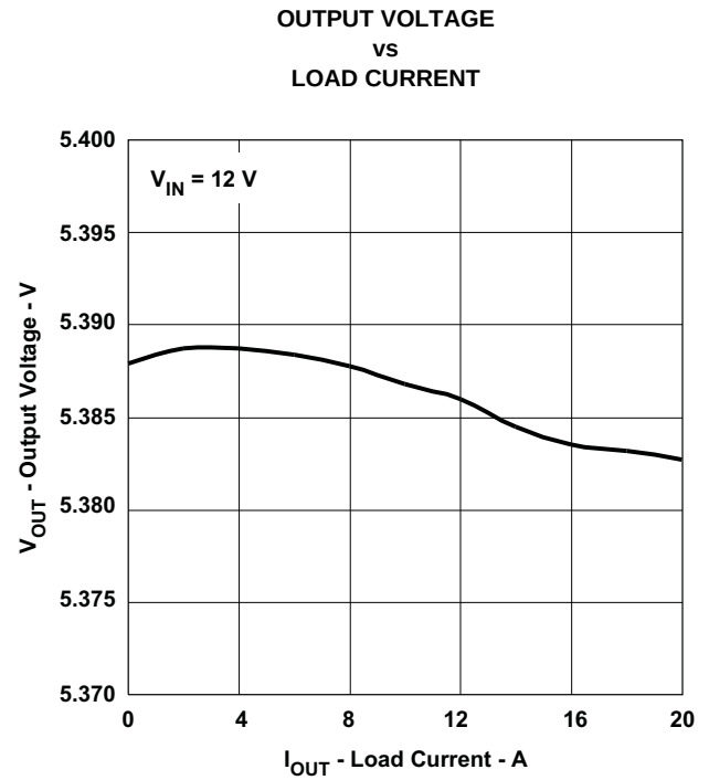
Figure 16. Load Regulation
