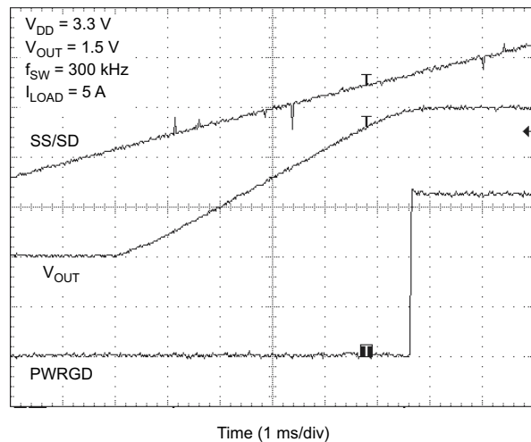
Figure 30. Start-Up Operation With Transient Comparators
