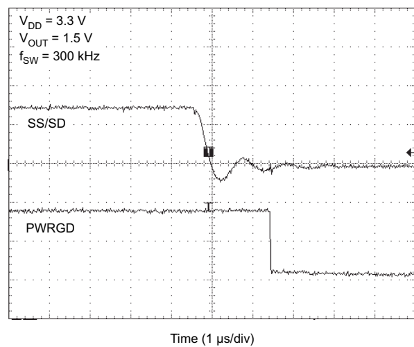
Figure 32. PWRGD Shutdown Operation
