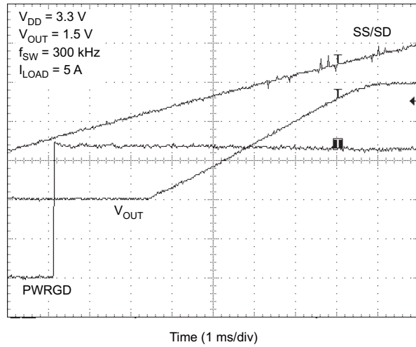
Figure 28. Start-Up Operation Without Transient Comparators
