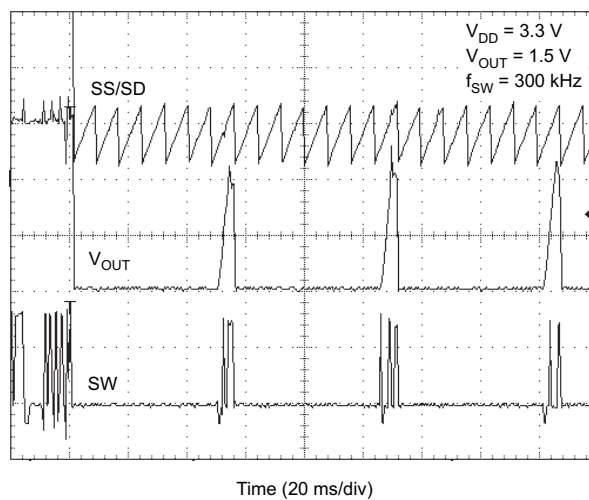
Figure 27. Output Current Fault Operation
