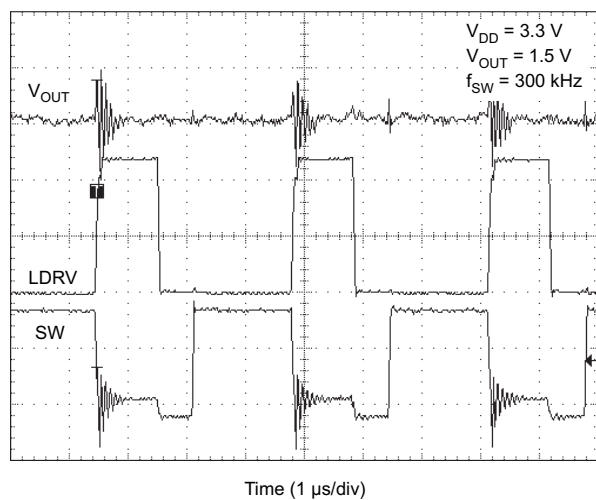
Figure 26. TPS40021 I_{\text{ZERO}} Detection – DCM
