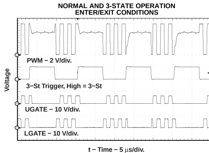
Figure 18. The 3-state upper threshold reverts to the 2-V level after the TPS28226 had been in 3-state for about 2.5 \mu\text{s} .
