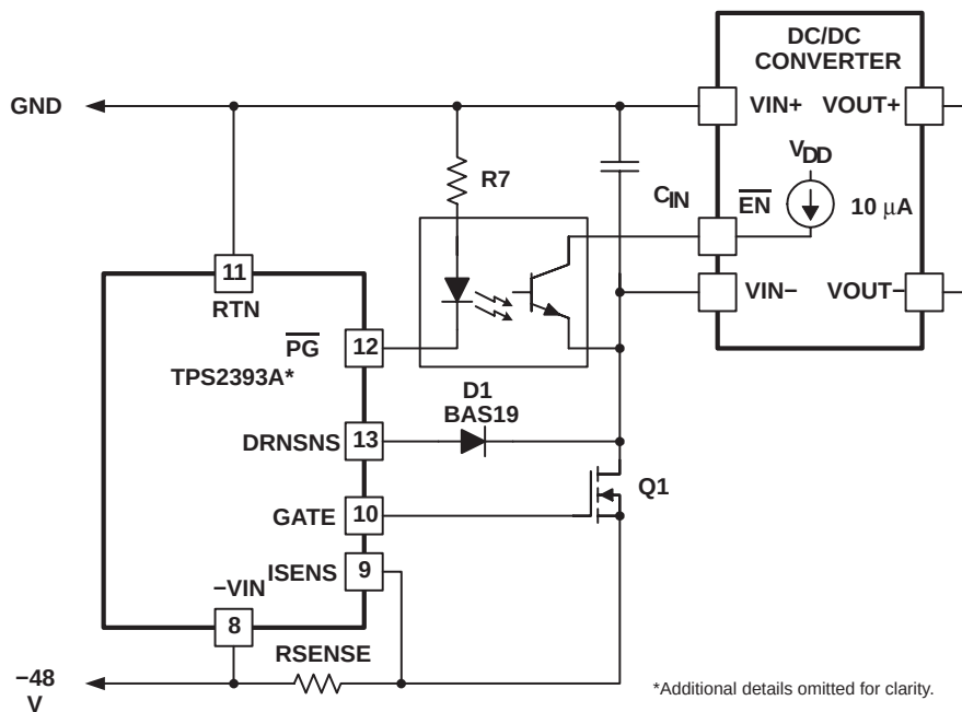
Figure 27. \overline{PG} Driving An Optocoupler
