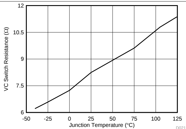
Figure 20. VC Switch Resistance vs Temperature
