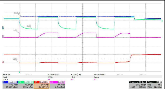
Figure 35. Converter Output Short and Recovery
