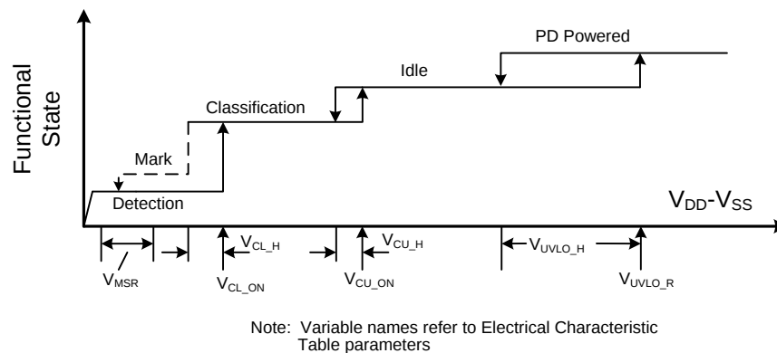
Figure 23. Threshold Voltages
