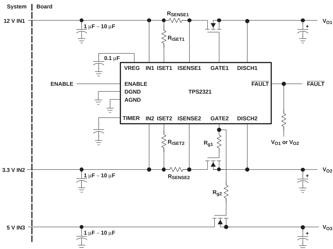
Figure 27. Three-Channel Application
