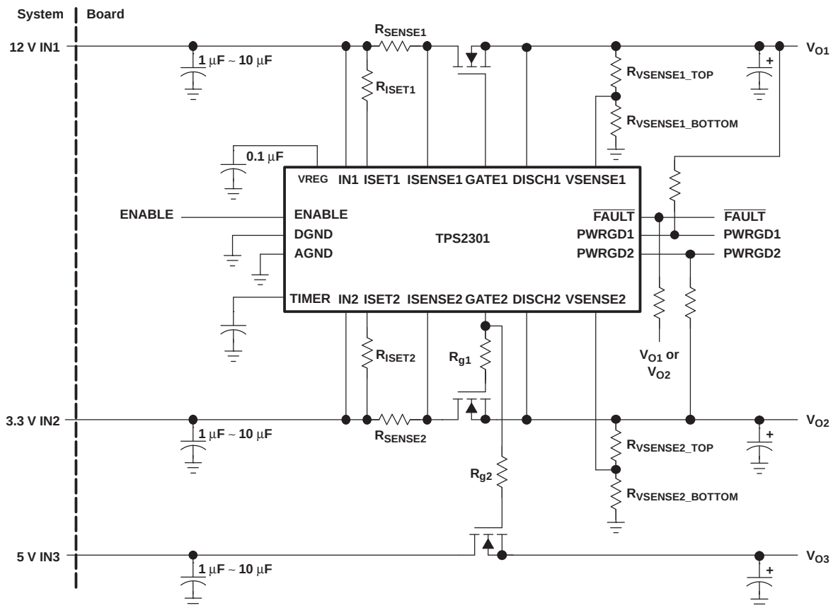
Figure 28. Three-Channel Application
