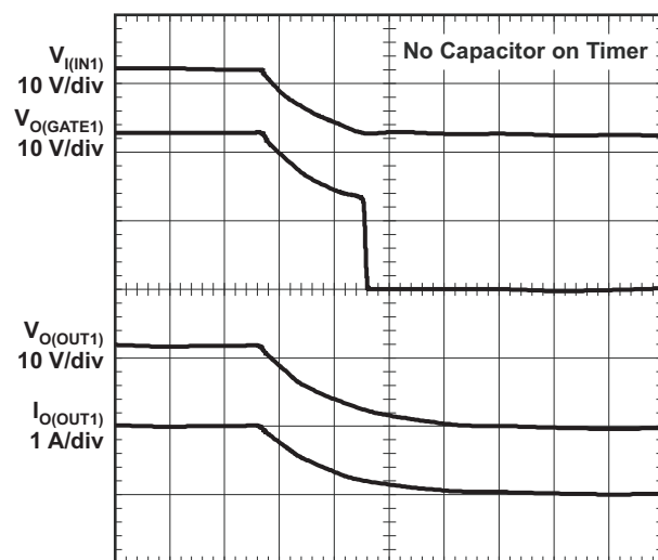
Figure 10. Channel 1 – Enabled Into Short Circuit
