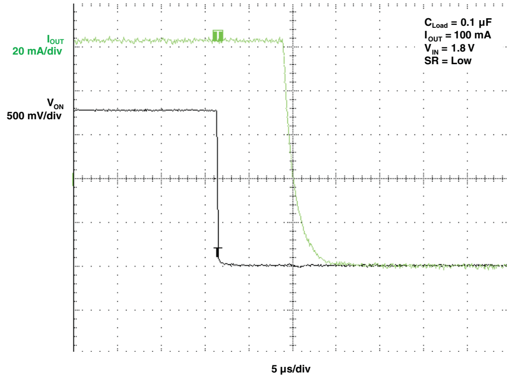
Figure 24. t_{OFF} Response
