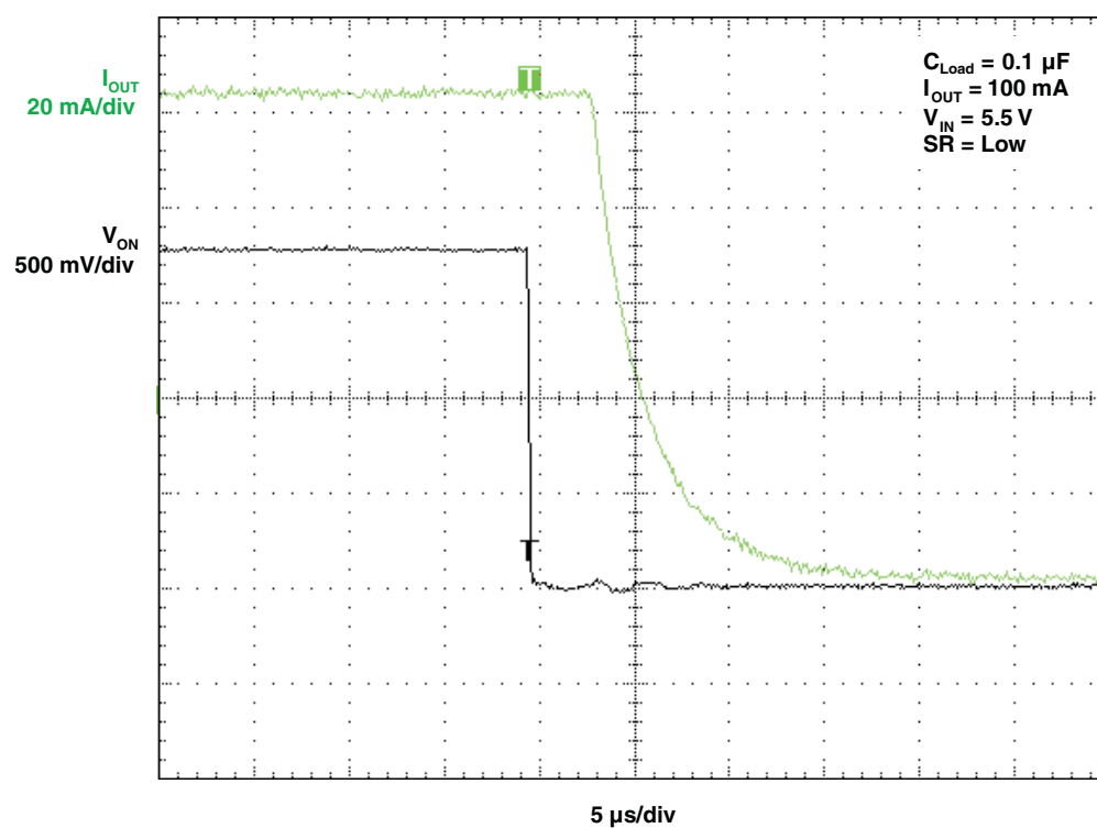
Figure 26. t_{OFF} Response
