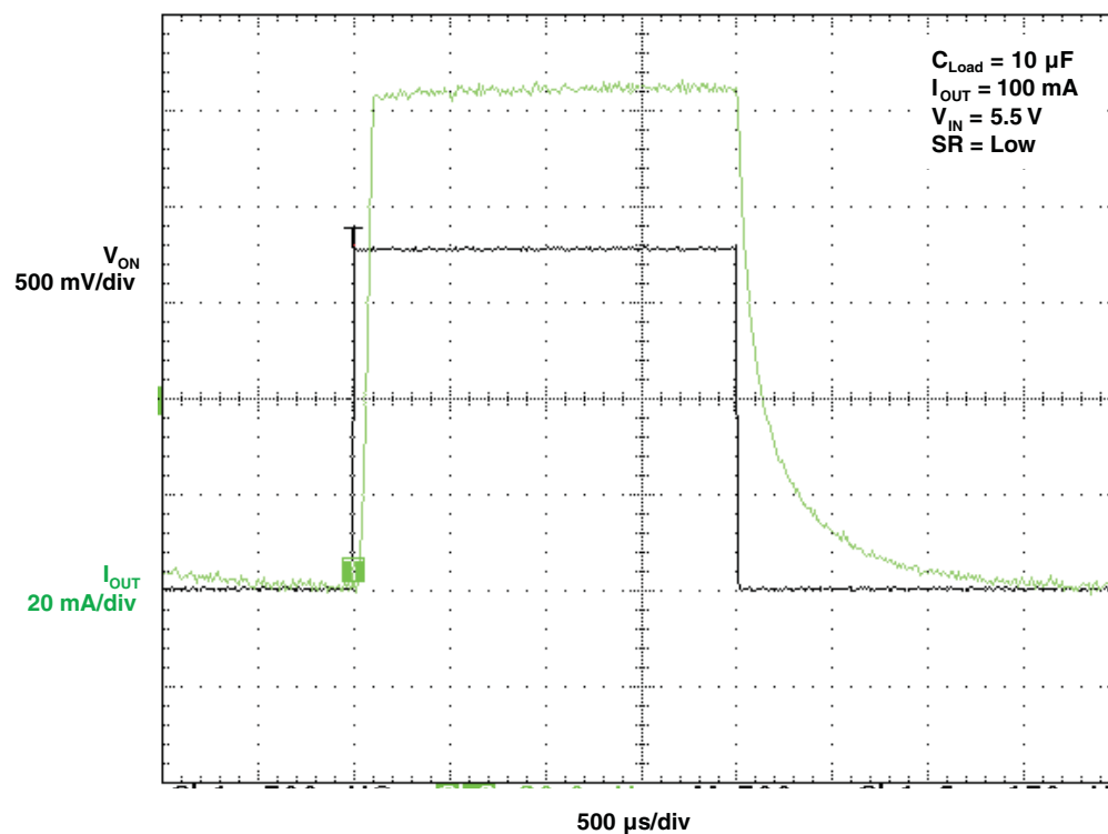
Figure 23. t_{ON} Response
