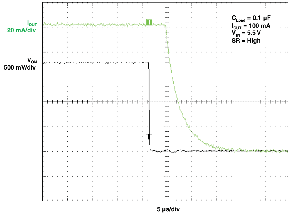
Figure 18. t_{OFF} Response
