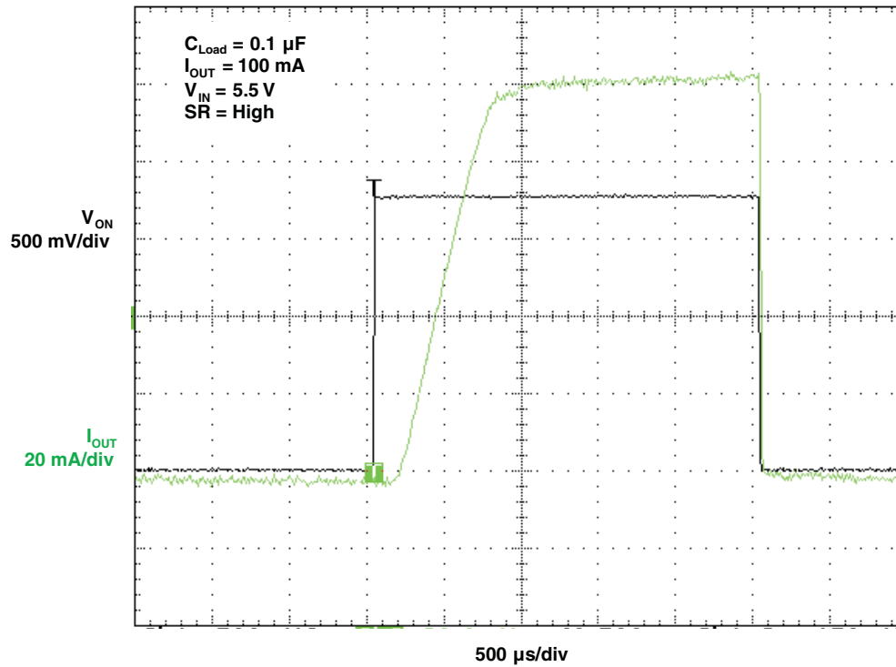
Figure 14. t_{ON} Response
