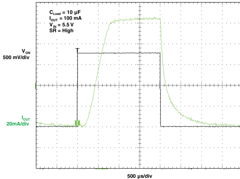
Figure 15. t_{ON} Response
