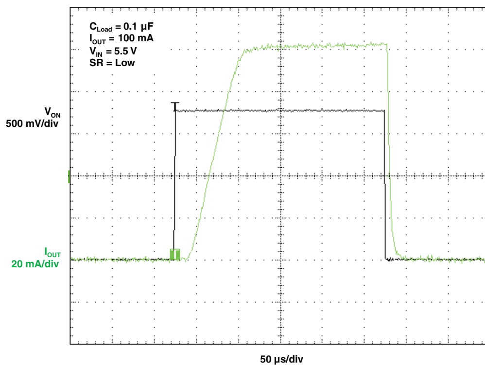
Figure 22. t_{ON} Response
