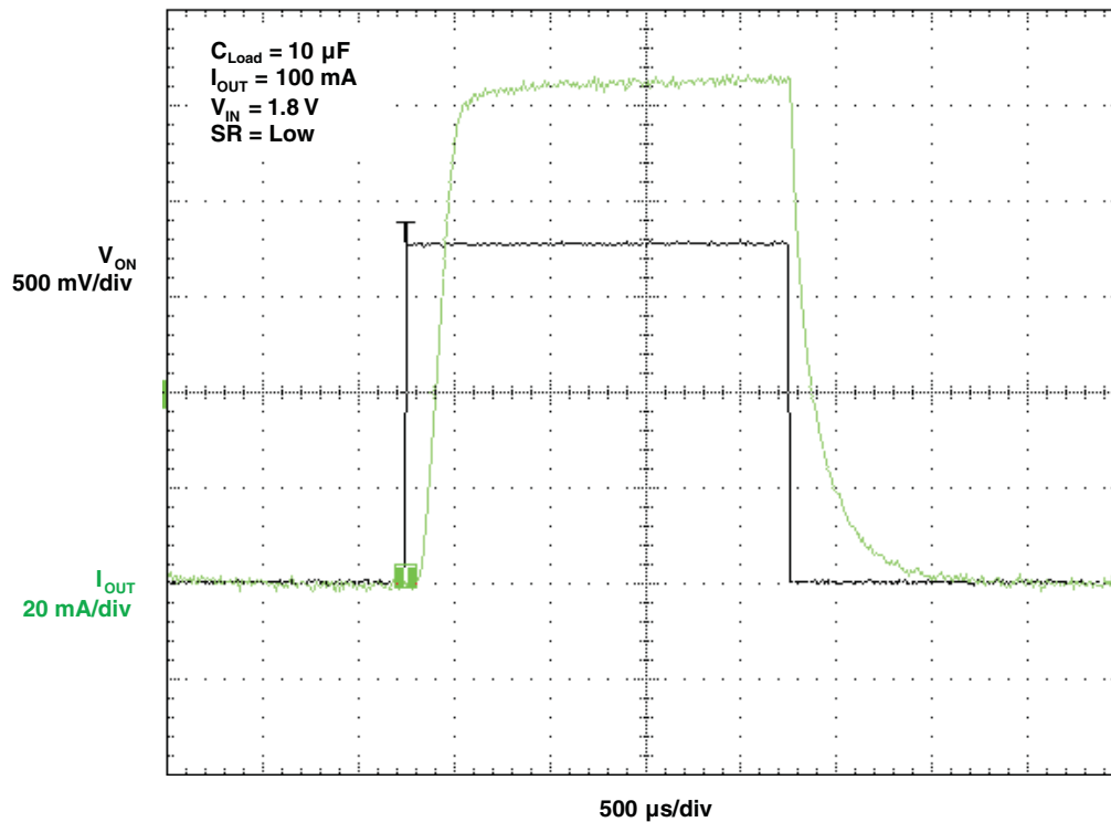
Figure 21. t_{ON} Response
