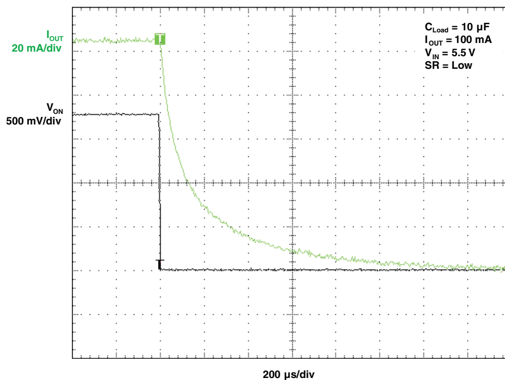
Figure 27. t_{OFF} Response
