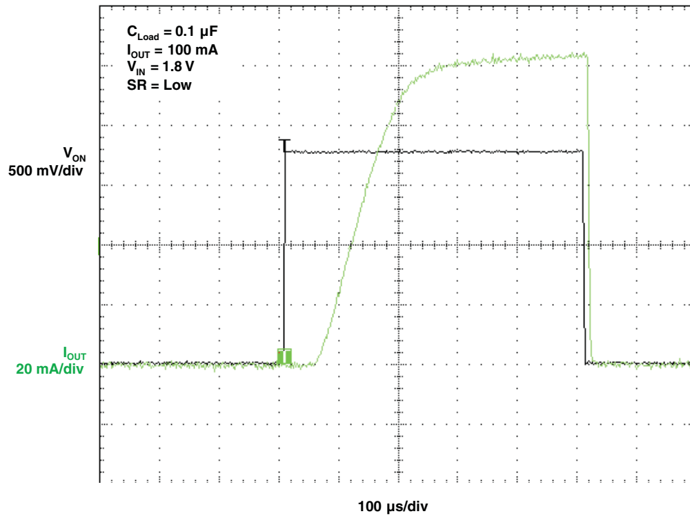
Figure 20. t_{ON} Response
