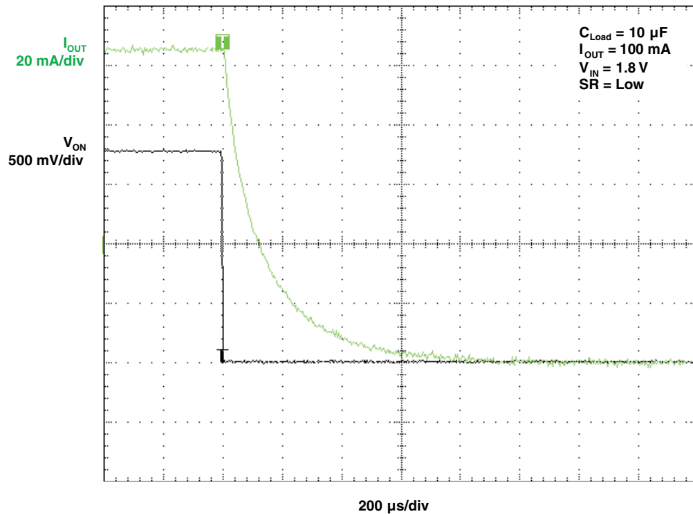
Figure 25. t_{OFF} Response
