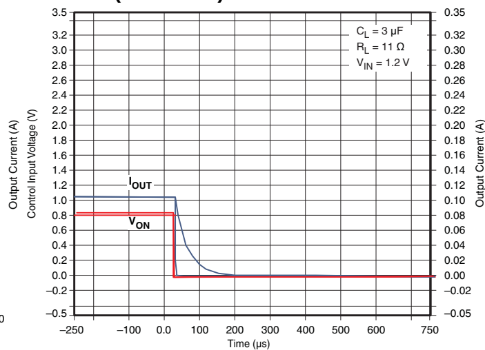
Figure 57. t_{OFF} Response
