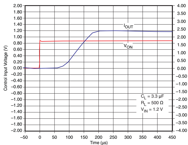
Figure 24. t_{ON} Response
