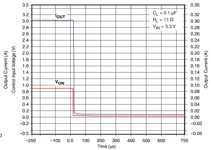
Figure 51. t_{OFF} Response
