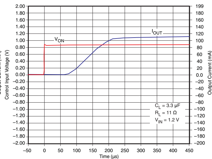
Figure 25. t_{ON} Response
