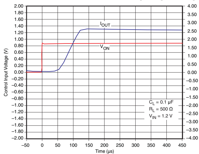
Figure 22. t_{ON} Response
