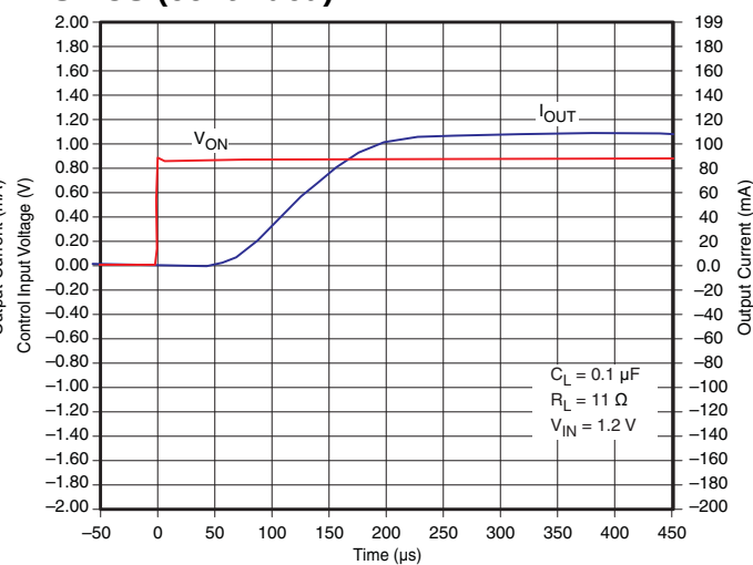
Figure 23. t_{ON} Response
