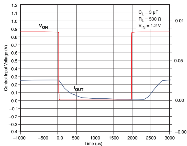
Figure 56. t_{OFF} Response
