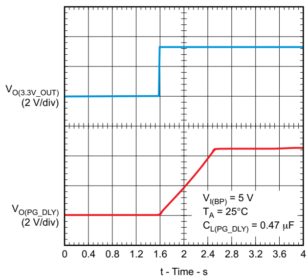
Figure 9. PG_DLY Rise Time With a 0.47-μF Capacitor
