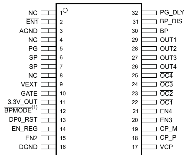
DAP Package (Top View)
