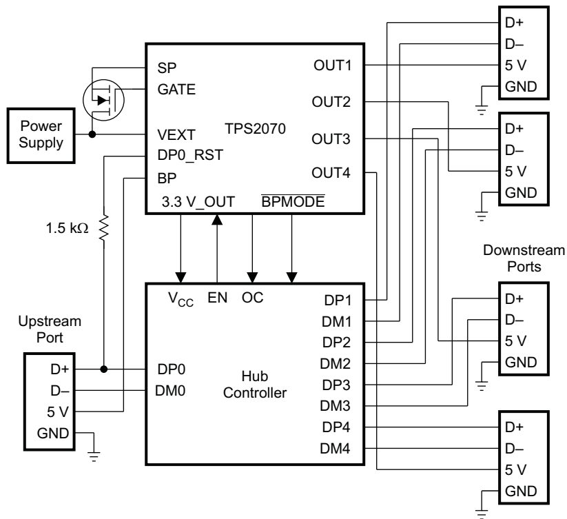
Simplified Hybrid-Hub Diagram (1)
