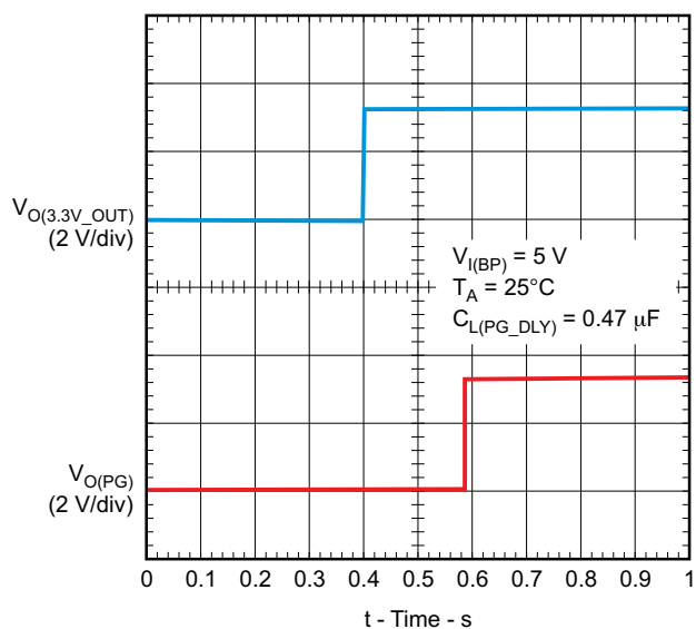
Figure 10. Turnon Delay (3.3V_OUT to PG)
