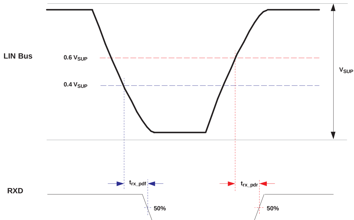
Figure 6. Propagation Delay
