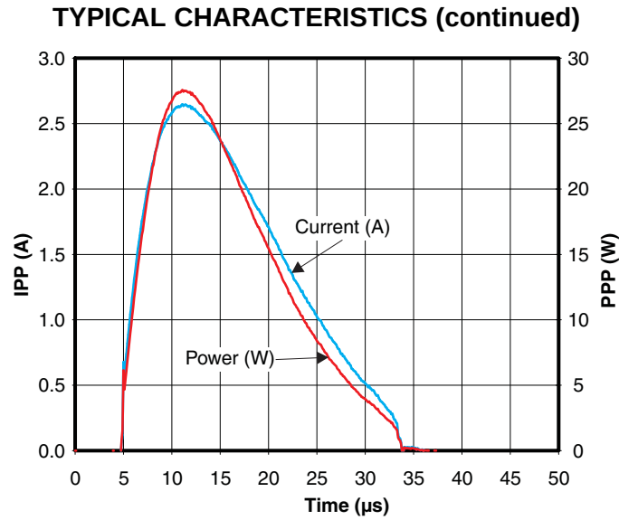
Figure 5. Pulse Waveform (8/20 μs Pulse)
