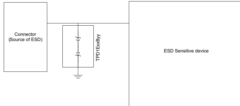
Figure 10. Application Schematic
