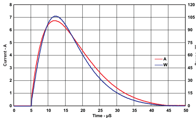
Figure 6. Positive Surge Waveform 8/20 \mu s
