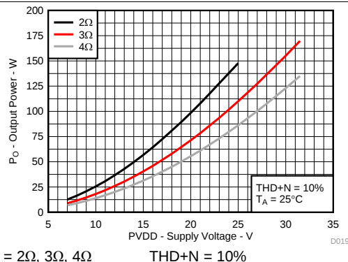
Figure 20. Output Power vs Supply Voltage
