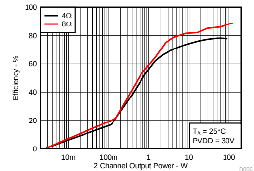
Figure 6. System Efficiency vs Output Power, AD-mode
