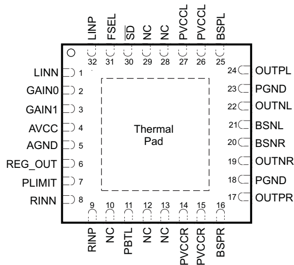
RHB (QFN) PACKAGE (TOP VIEW)
