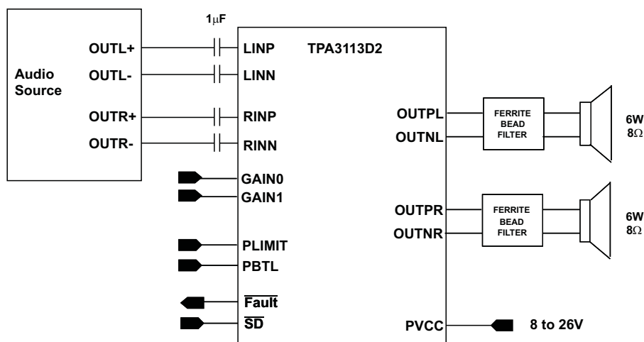
Figure 1. TPA3113D2 Simplified Application Schematic
