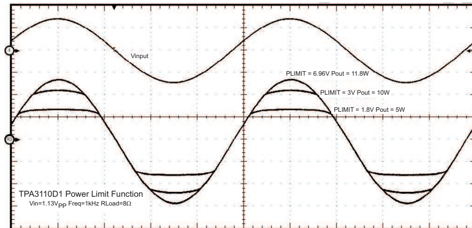
Figure 32. PLIMIT Circuit Operation
