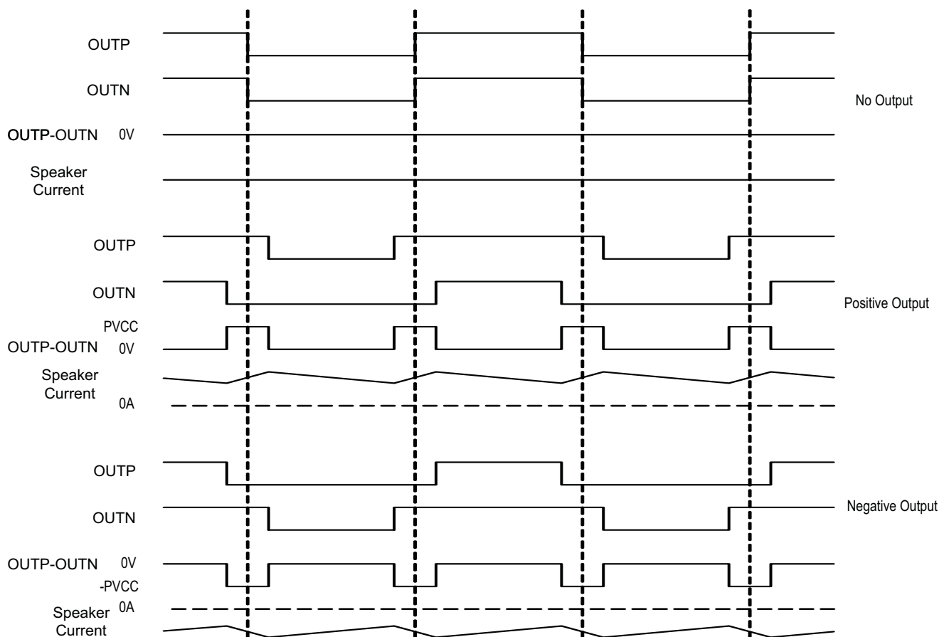
Figure 35. The TPA3113D2 Output Voltage and Current Waveforms Into an Inductive Load
