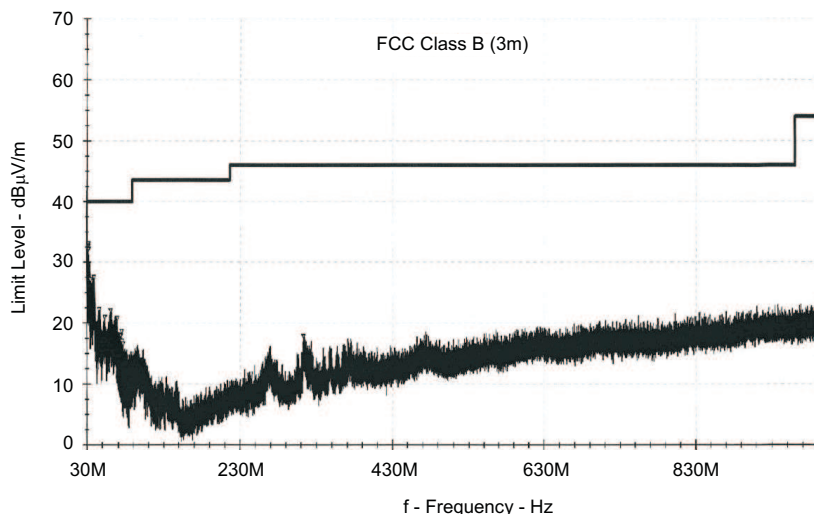
Figure 36. TPA3113D2 EMC spectrum with FCC Class B Limits
