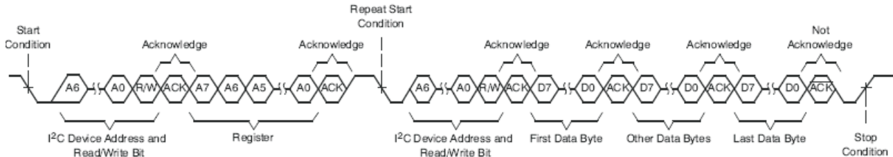
Figure 46. Multi-Byte Read Transfer
