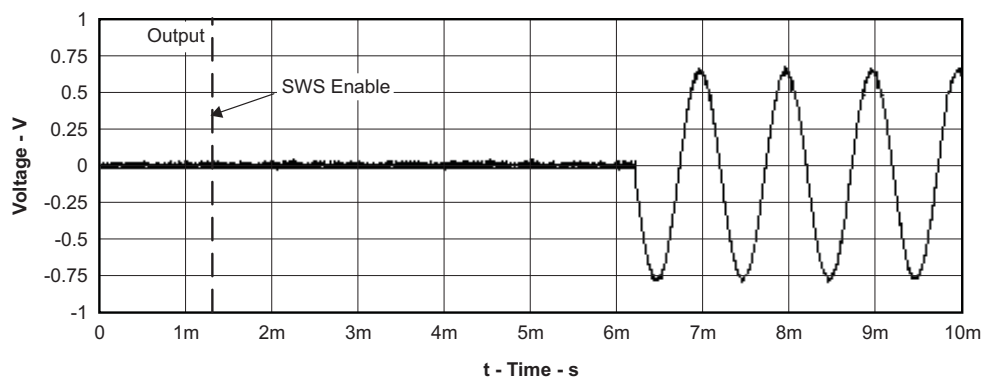
Figure 24. Startup Time
