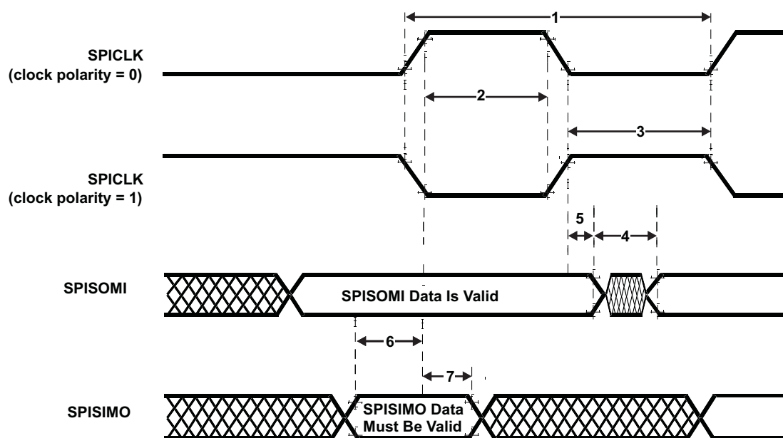
Figure 5-20. SPI Slave Mode External Timing (CLOCK PHASE = 1)
