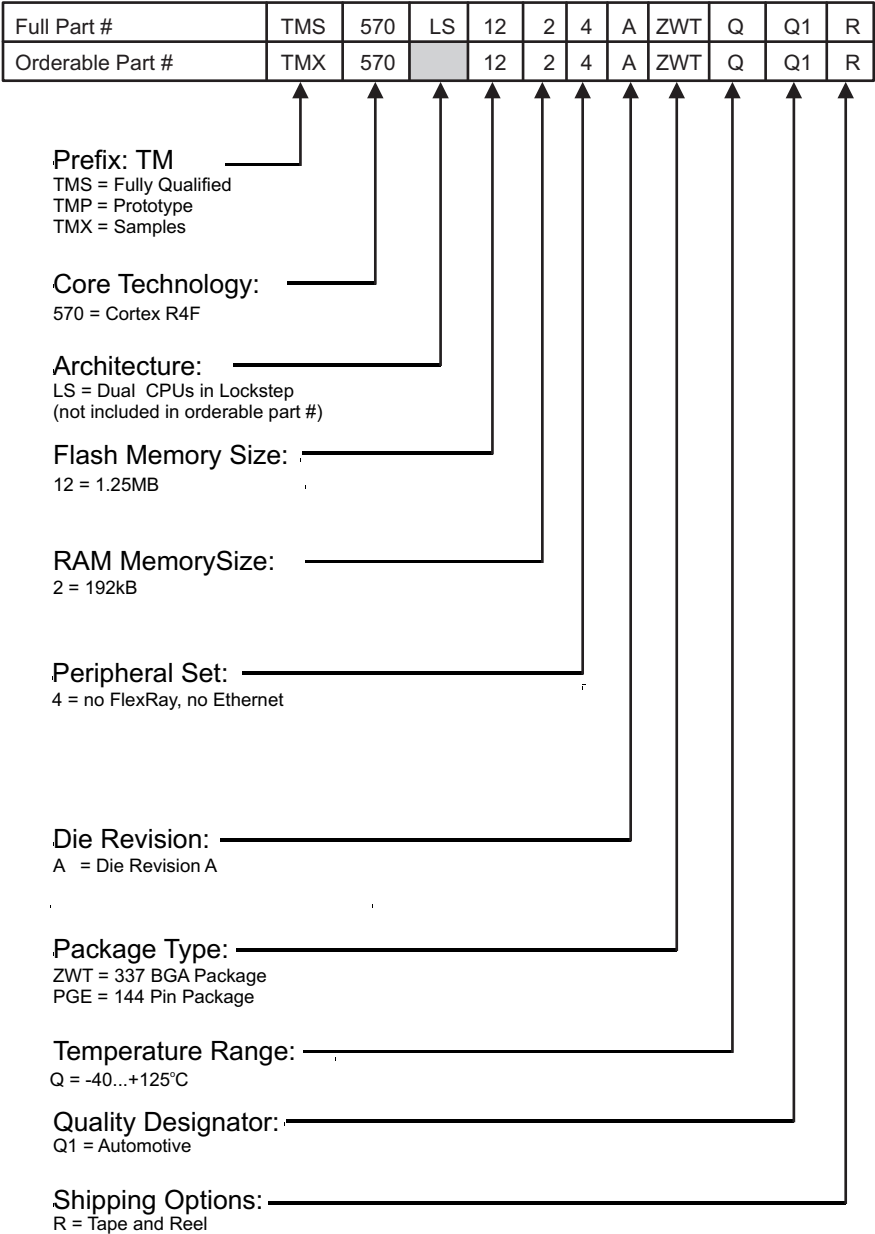
Figure 6-1. TMS570LS1224 Device Numbering Conventions
