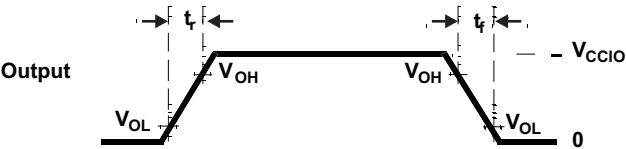
Figure 3-3. CMOS-Level Outputs
