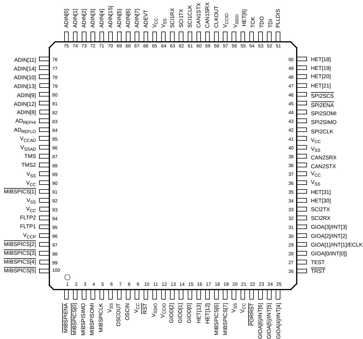
TMS470R1VF4B8 100-PIN PZ PACKAGE (TOP VIEW)
