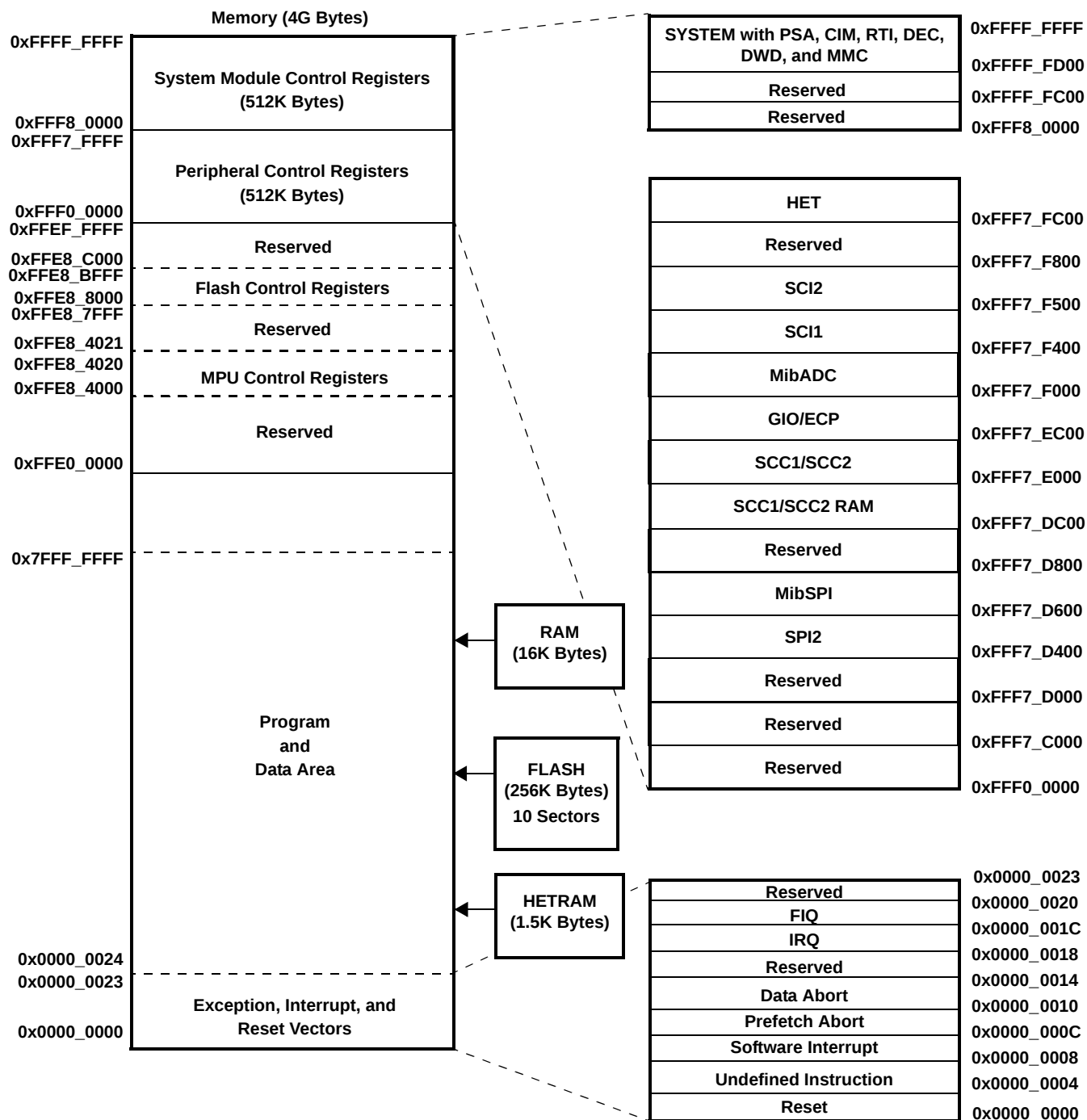
Figure 1. TMS470R1VF4B8 Memory Map
