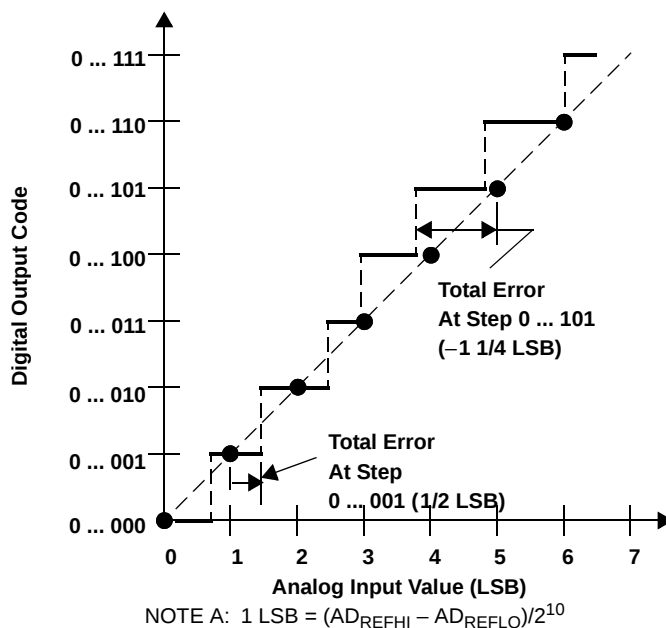
Figure 21. Absolute Accuracy (Total) Error
