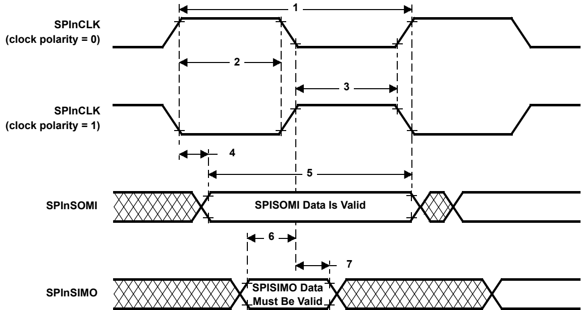
Figure 13. SPIn Slave Mode External Timing (CLOCK PHASE = 0)
