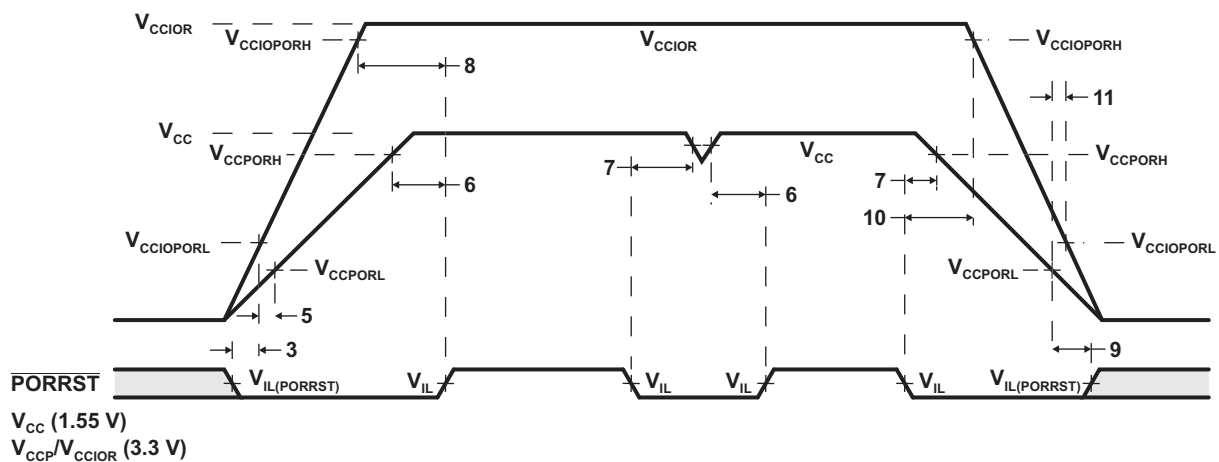
Figure 5-1. \overline{\text{PORRST}} Timing Diagram
