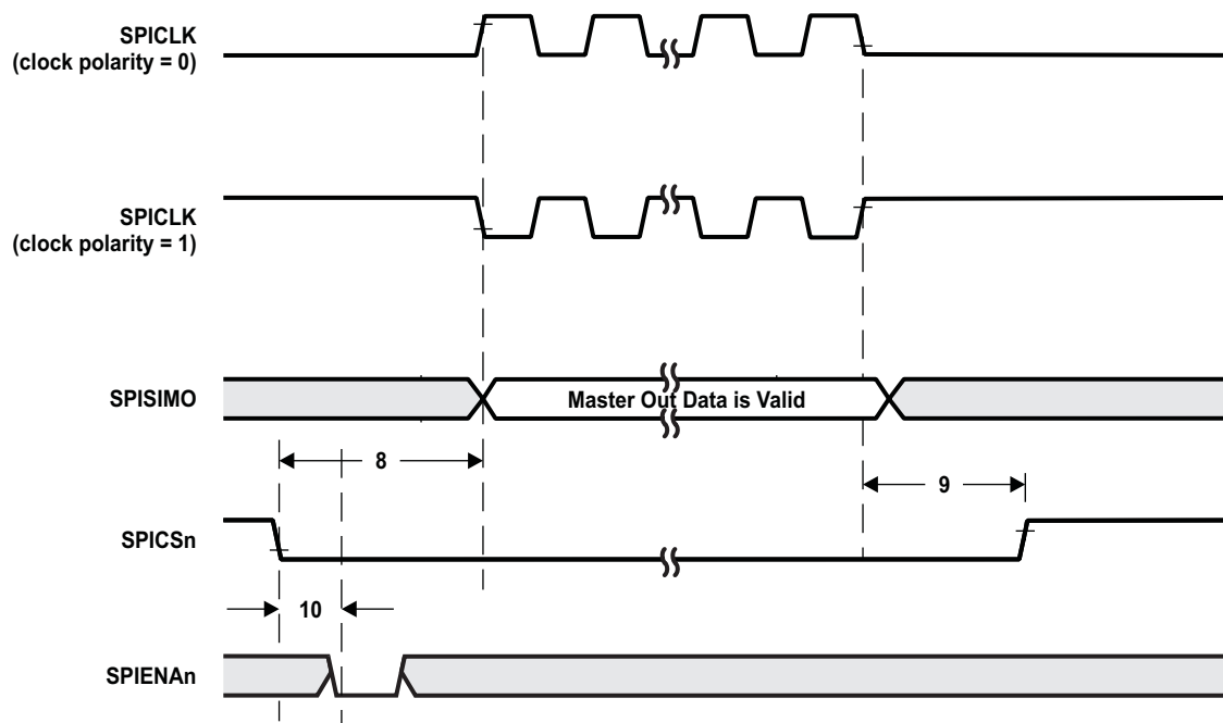
Figure 5-14. SPI Master Mode Chip Select Timing (CLOCK PHASE = 0)
