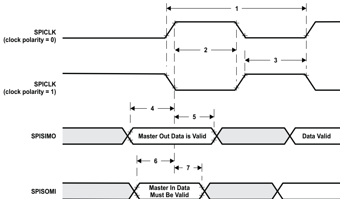
Figure 5-15. SPI Master Mode External Timing (CLOCK PHASE = 1)
