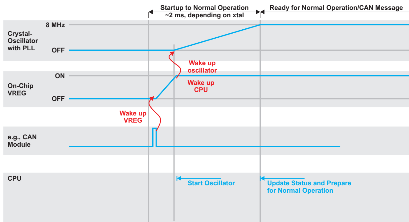
Figure 5-4. Wake Up From Sleep Mode
