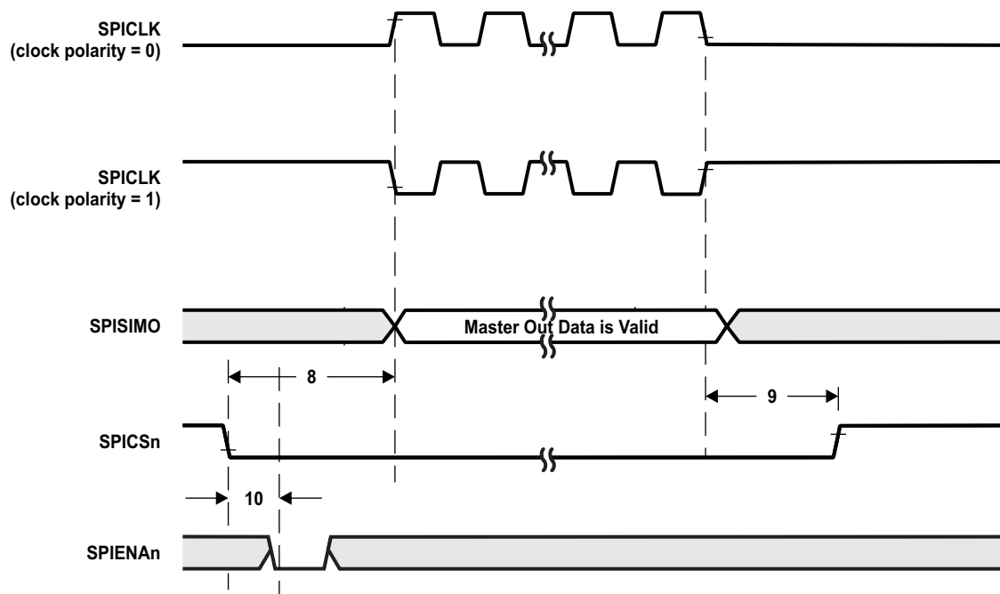
Figure 5-16. SPI Master Mode Chip Select timing (CLOCK PHASE = 1)
