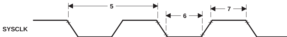
Figure 18. SYSCLK Timing
