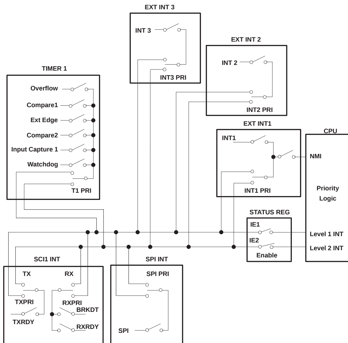
Figure 4. Interrupt Control
