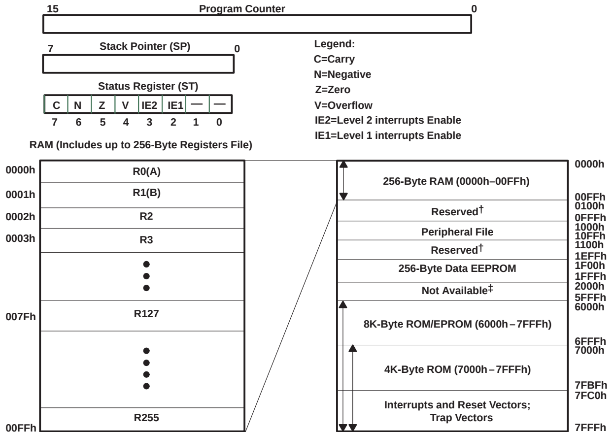
Figure 1. Programmer's Model
