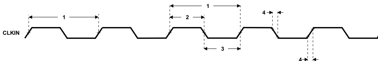
Figure 6-7. CLKIN Timing
