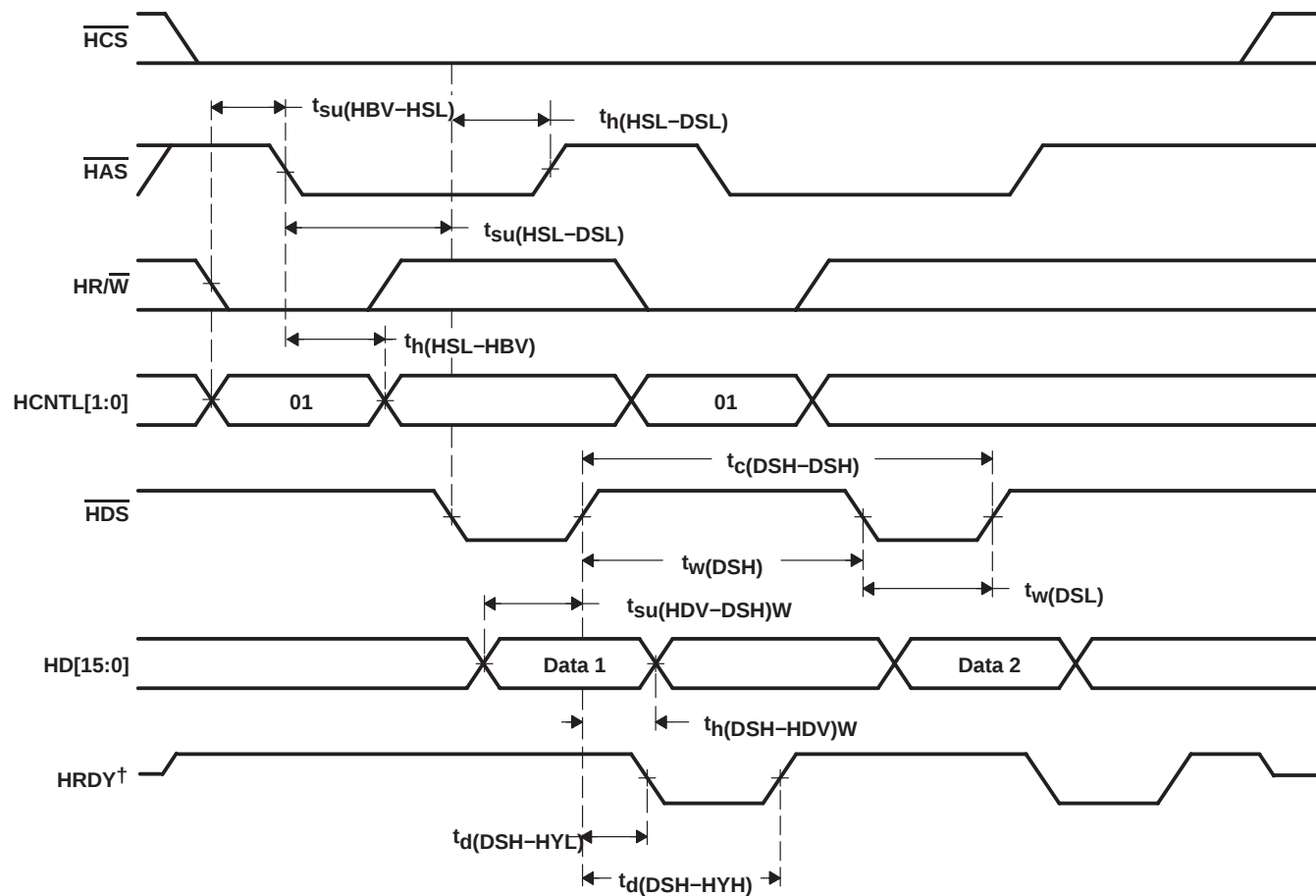
Figure 5–15. Multiplexed Write Timings Using \overline{HAS}
