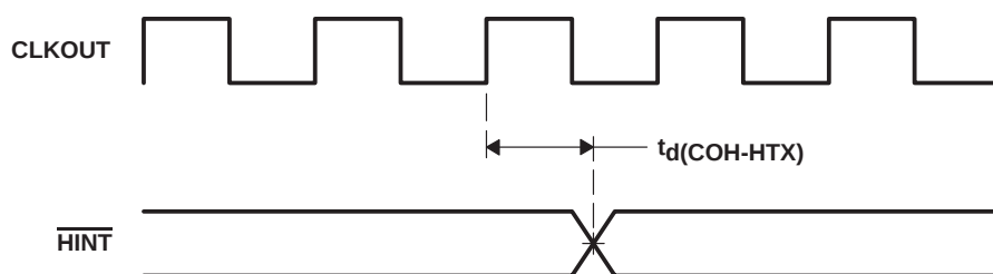
Figure 37. \overline{\text{HINT}} Timing
