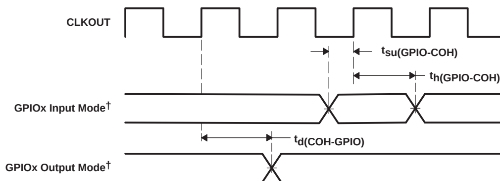
Figure 6-30. GPIOx † Timings
