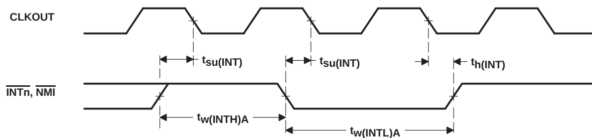
Figure 6-15. Interrupt Timing
