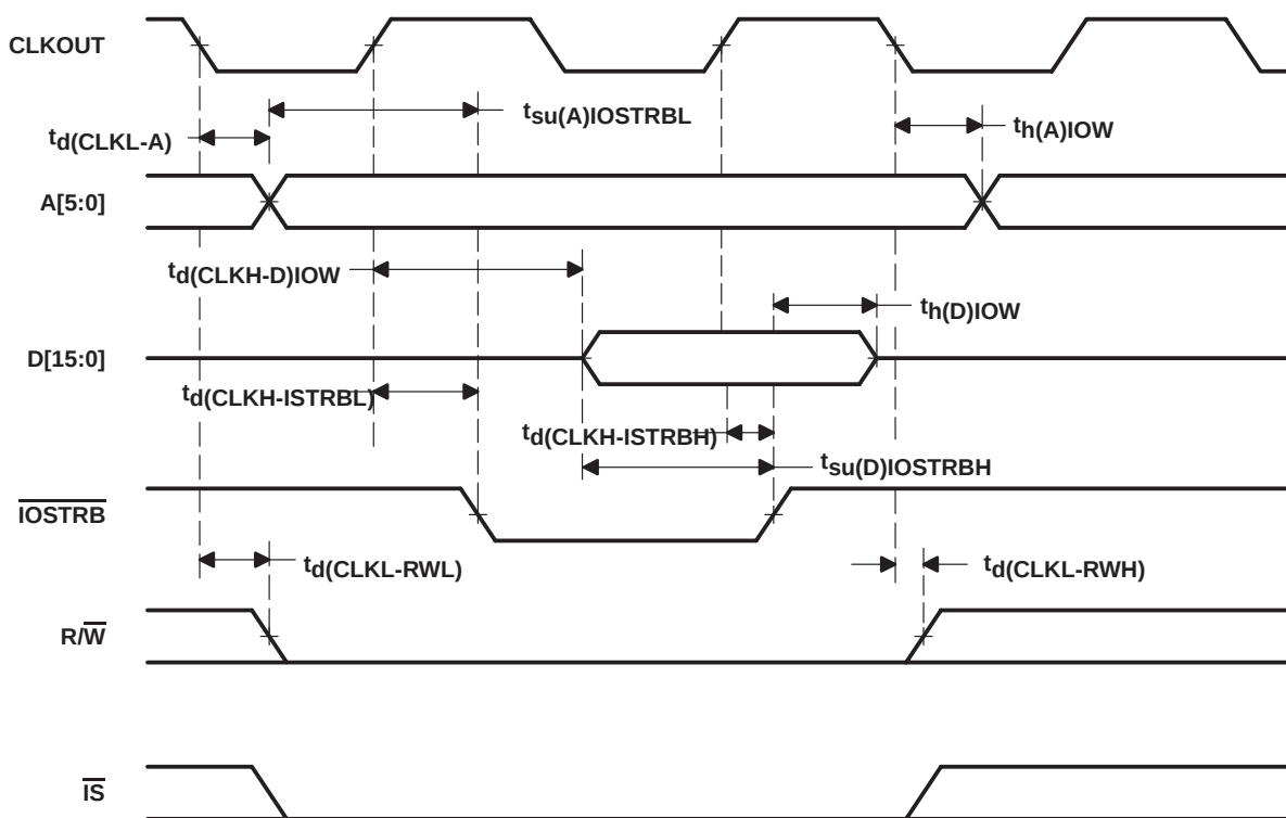
Figure 6–8. Parallel I/O Port Write
