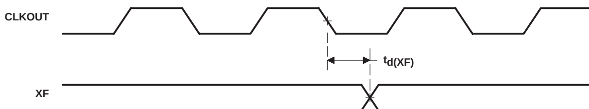
Figure 6–18. XF Timing
