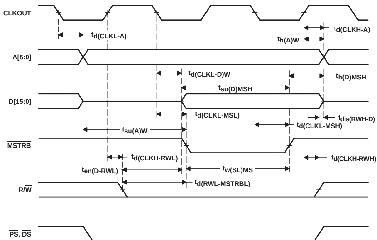
Figure 6–6. Memory Write
