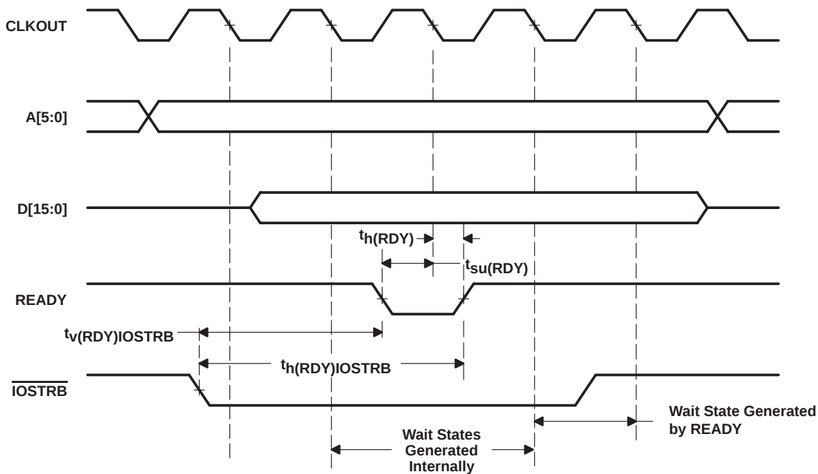
Figure 6-12. I/O Write With Externally Generated Wait States
