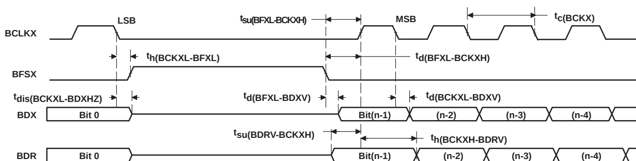
Figure 6–24. McBSP Timing as SPI Master or Slave: CLKSTP = 11b, CLKXP = 0
