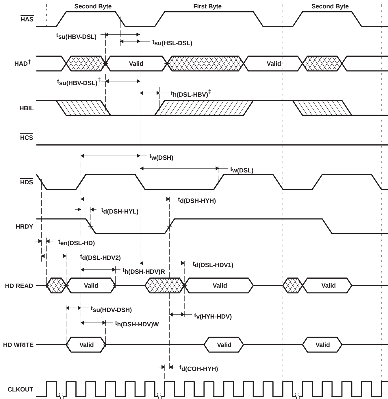
Figure 6-27. Using \overline{HDS} to Control Accesses ( \overline{HCS} Always Low)
