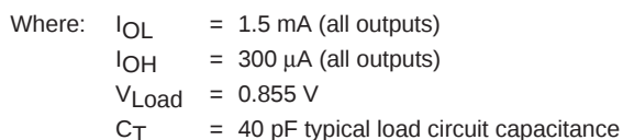
Figure 6-1. 1.8-V Test Load Circuit
