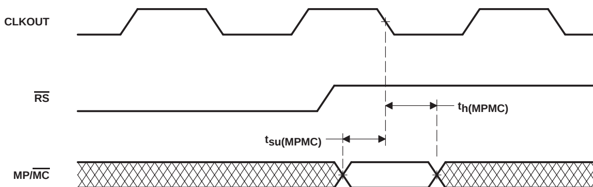
Figure 6-16. \text{MP}/\overline{\text{MC}} Timing
