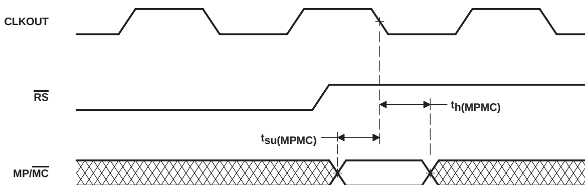
Figure 4-16. \text{MP}/\overline{\text{MC}} Timing
