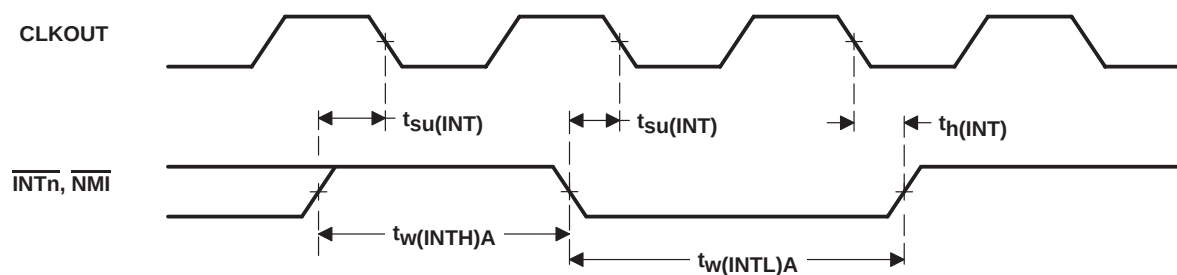
Figure 4-15. Interrupt Timing
