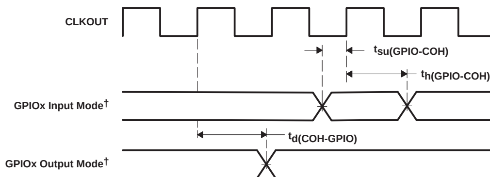
Figure 4-30. GPIOx ^\dagger Timings
