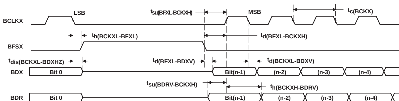
Figure 4–24. McBSP Timing as SPI Master or Slave: CLKSTP = 11b, CLKXP = 0
