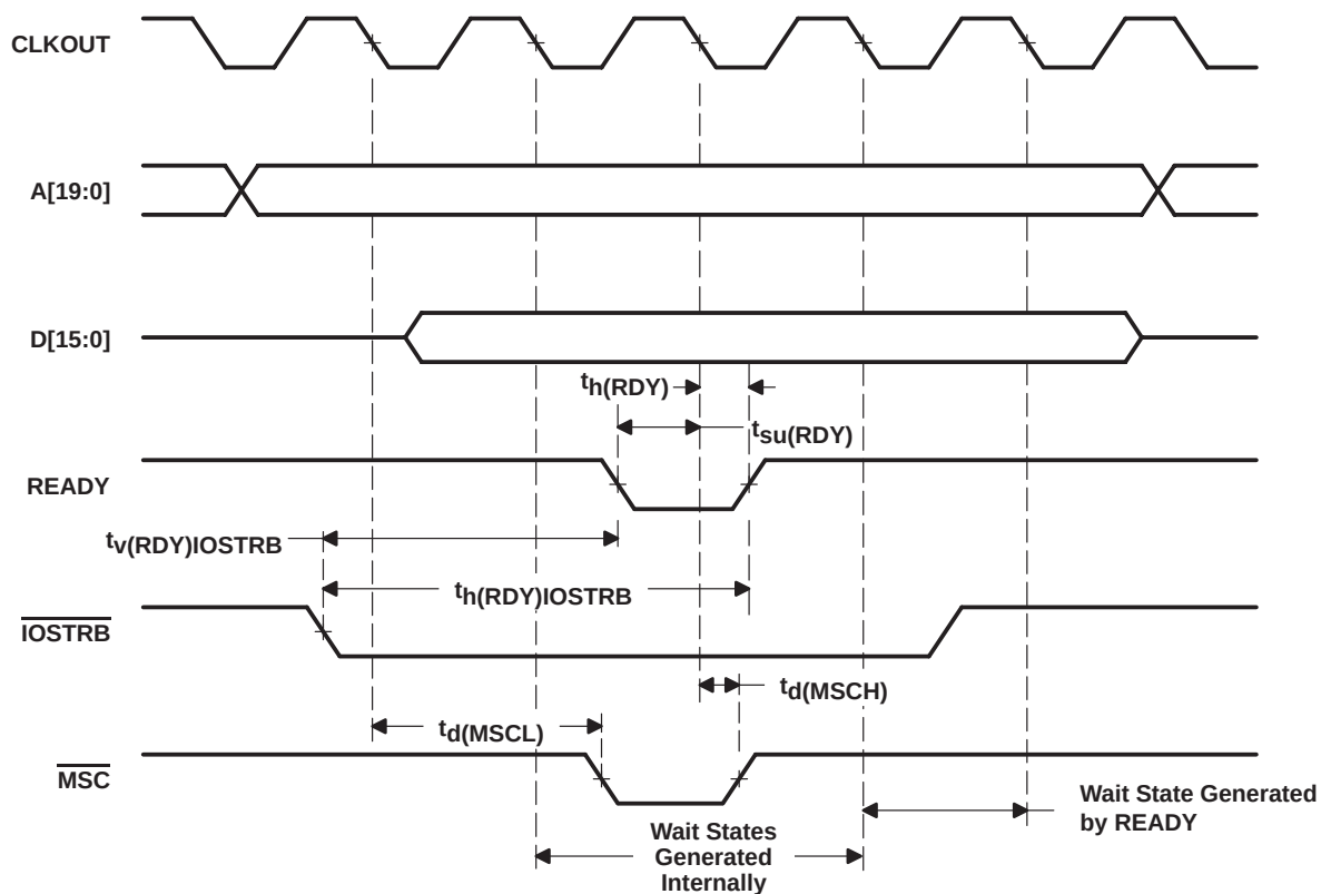
Figure 4-12. I/O Write With Externally Generated Wait States
