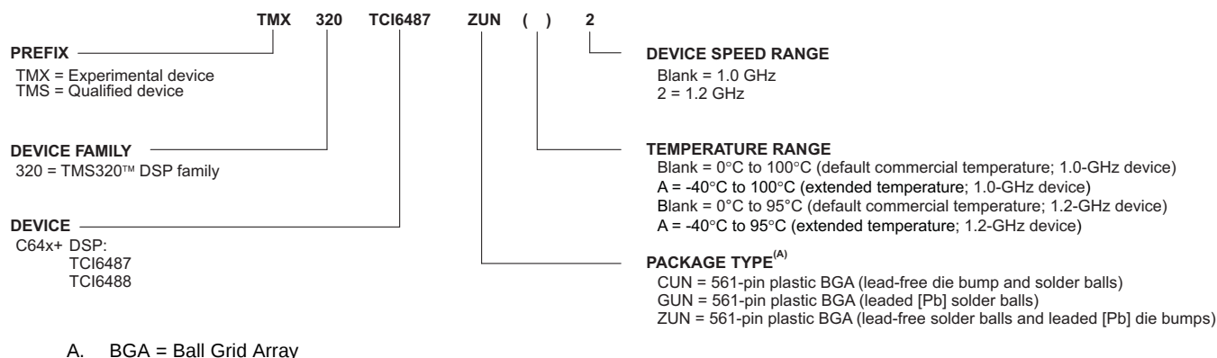
Figure 2-11. TMS320C64x+™ DSP Device Nomenclature (including TMS320TCI6487/8 DSP)
