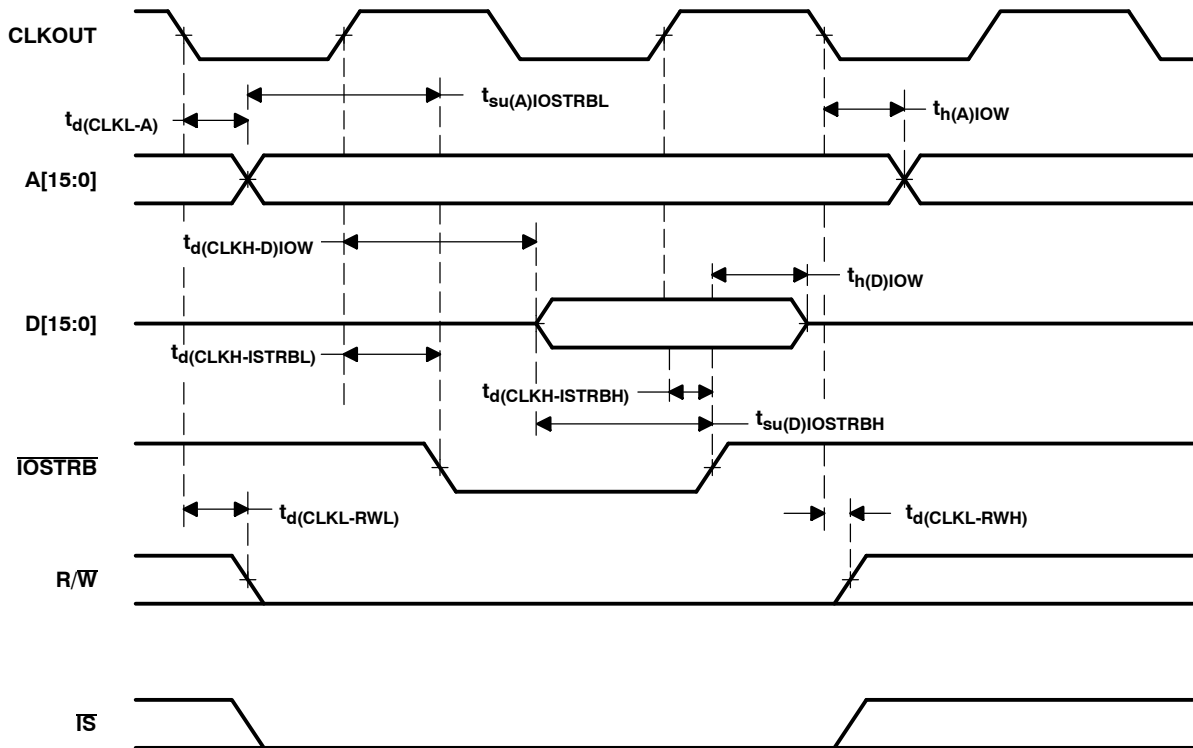
Figure 8. Parallel I/O Port Write ( \overline{IOSTRB} = 0 )
